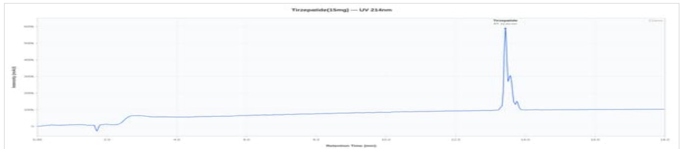
GLP- 2 TZ 15mg - BPB-2610-001: UV Chromatogram
